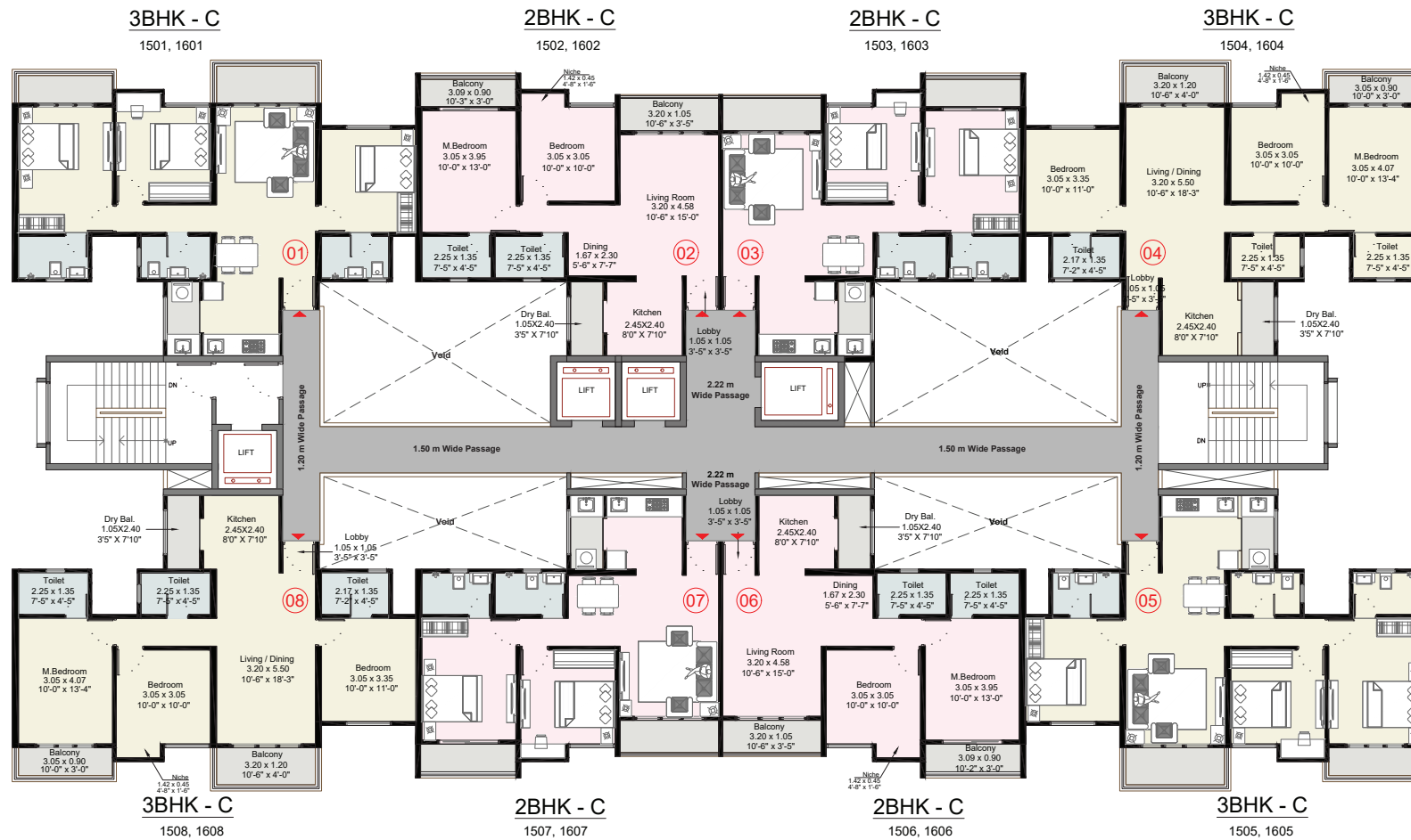
15TH & 16TH FLOOR PLAN
