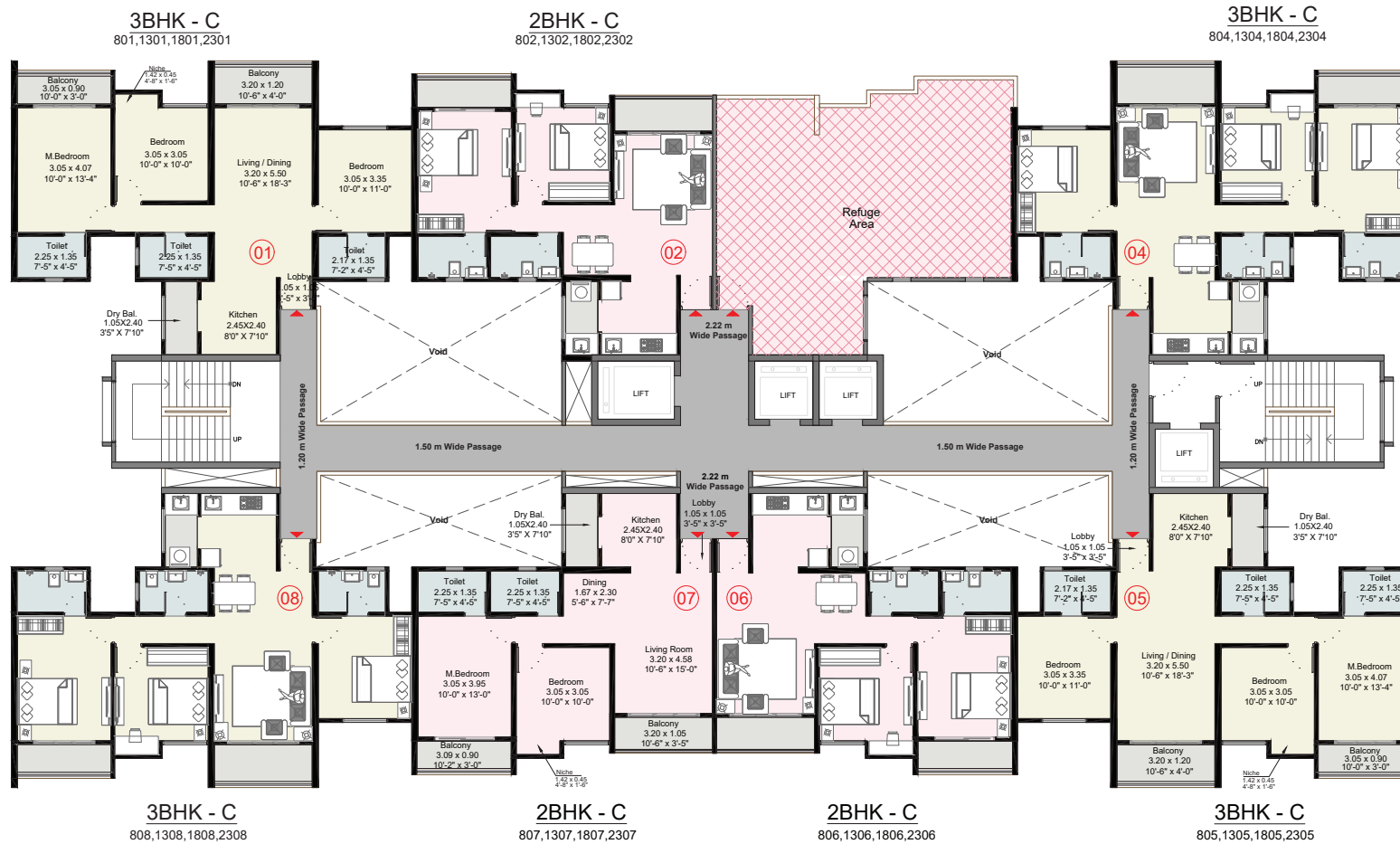
8,13,18,23RD REFUGE FLOOR PLAN
