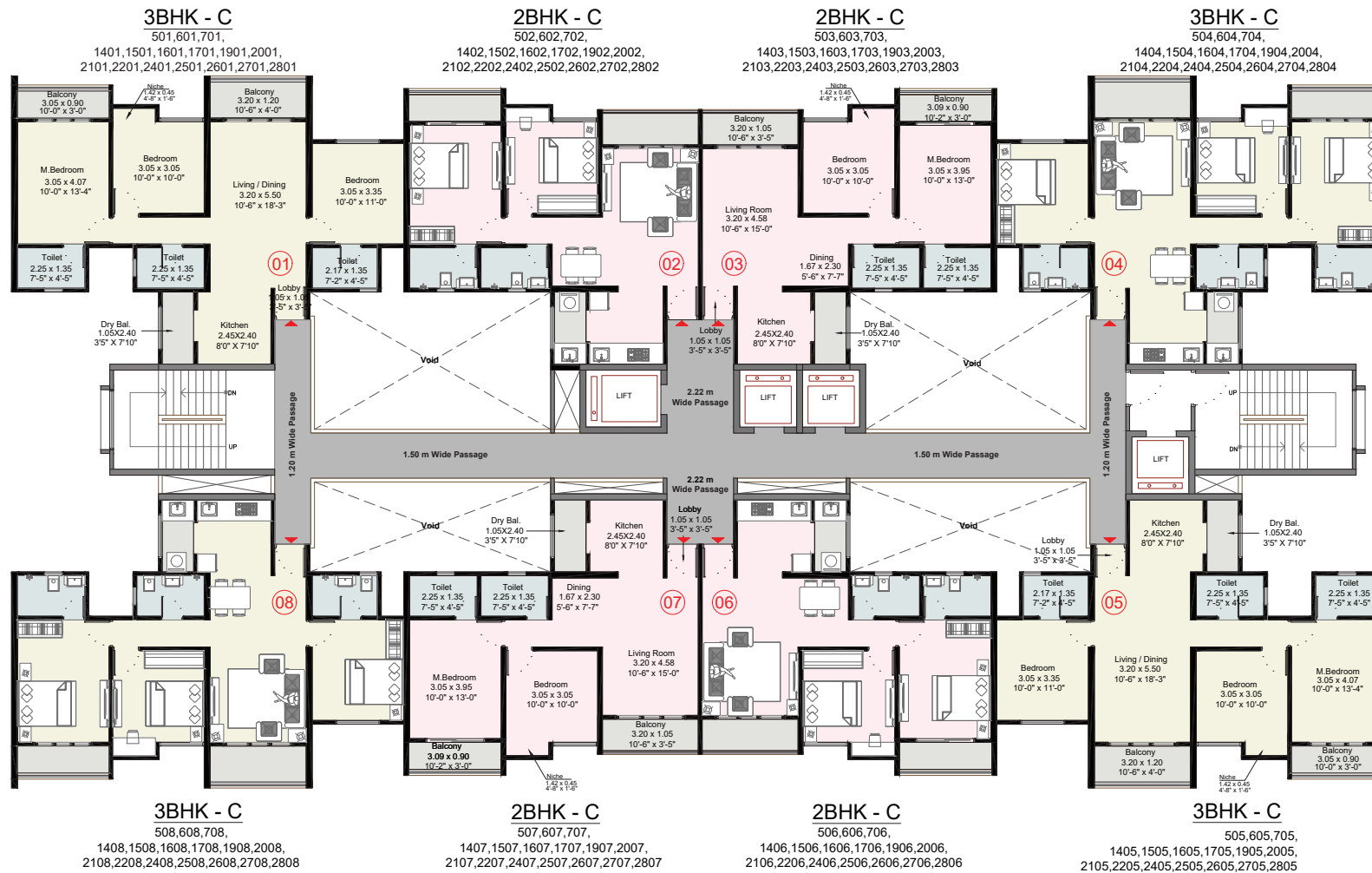
TYPICAL FLOOR PLAN- 5,6,7,14,15,16,17,19,20,21,22,24,25,26,27,28TH FLOOR
